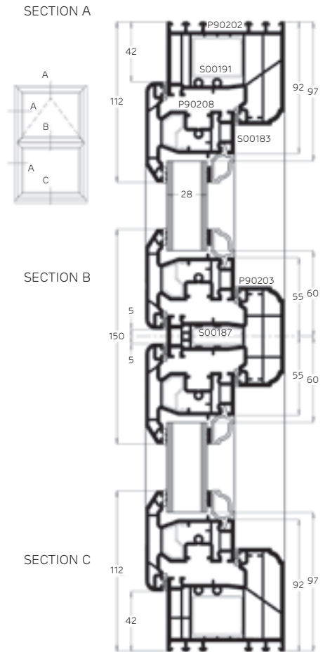
Storm 72mm Outer Frame Large
