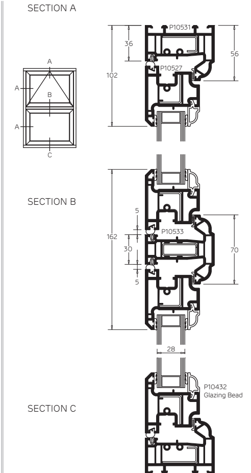
CLARITY 56mm Flush Outer Frame Slim
