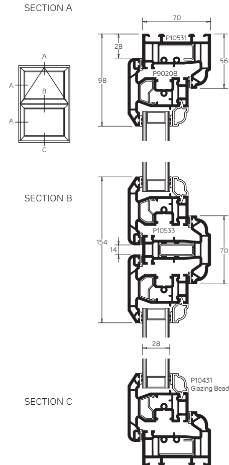
CLARITY 56mm Storm Outer Frame Slim
