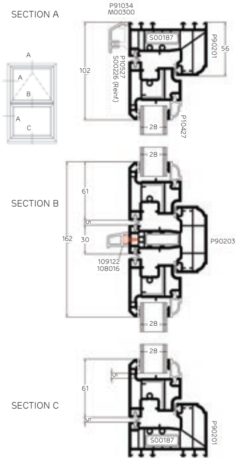
Flush 56mm Outer Frame Slim
