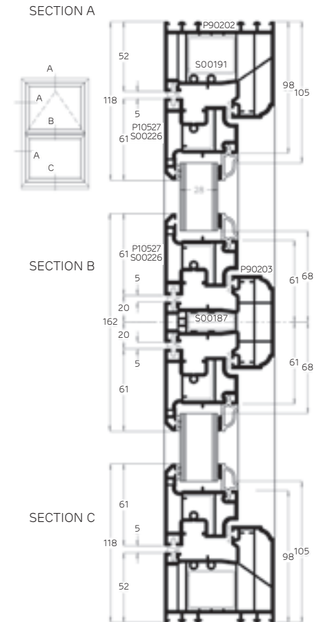
Flush 72mm Outer Frame Large
