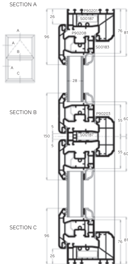
Storm 56mm Outer Frame Slim
